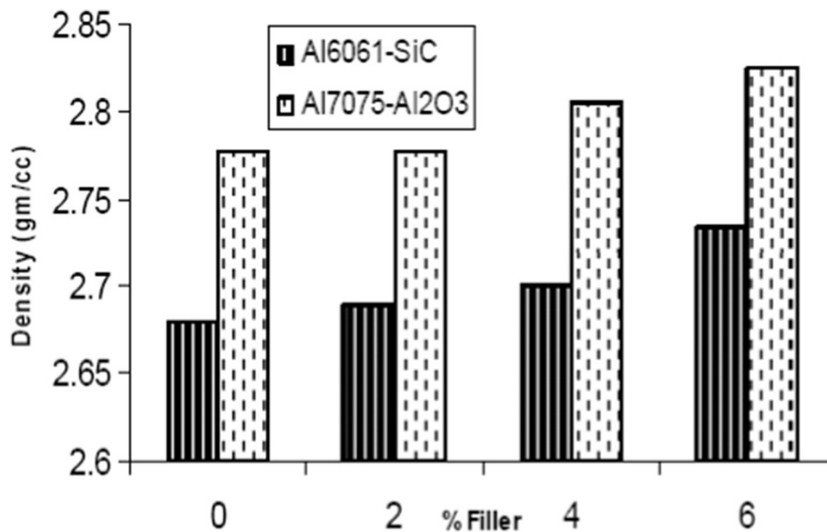
Figure 5 Density of Al6061-SiC and Al7075-Al2O3 composites (Veeresh Kumar et al. 2010).
