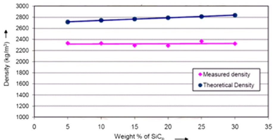
Figure 6 Comparison between measured and theoretical densities of un-sintered Al-SiCp composites (Purohit et al. 2012).
